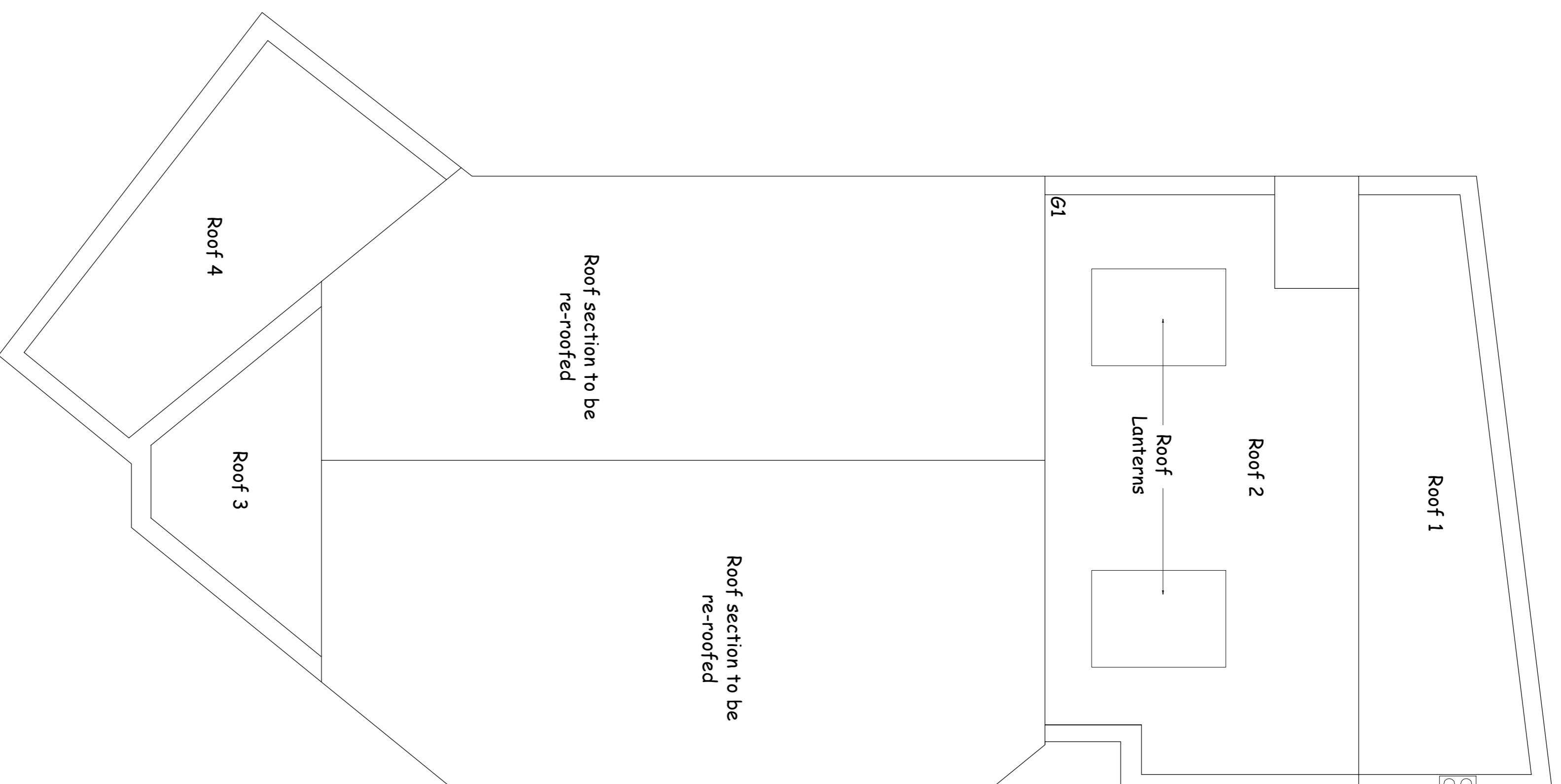
Proposed Roof Plan
